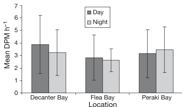
Fig. 3. Mean daytime and nighttime detection rates ( \pm 95\% CI) of Cephalorhynchus dolphins at Decanter, Flea and Peraki Bays, New Zealand. DPM: detection-positive minutes
