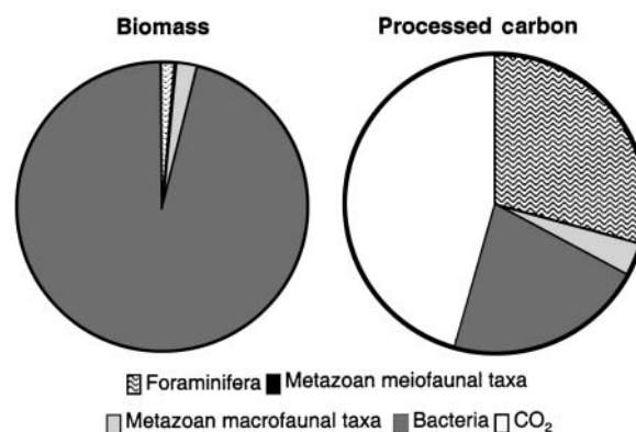
Fig. 2. Proportional division of biomass and processed carbon among the different benthic compartments. Fauna are those retained on a 300 \mu\text{m} sieve and values are average of the 2 experimental chambers
