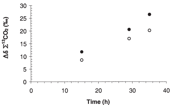
Fig. 1. ^{13}\text{C} -enrichment of total inorganic carbon ( \Delta\delta\Sigma^{13}\text{CO}_2 ) versus time. Values from experimental chambers, ALBEX 2 (○) and ALBEX 3 (●)
