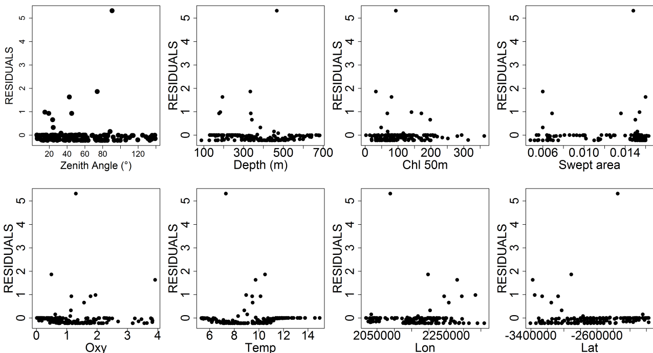
Figure S2: Pearson residuals plotted against all covariates for the Negative binomial GAM applied to the catch rates of M. paradoxus of all four size groups.
