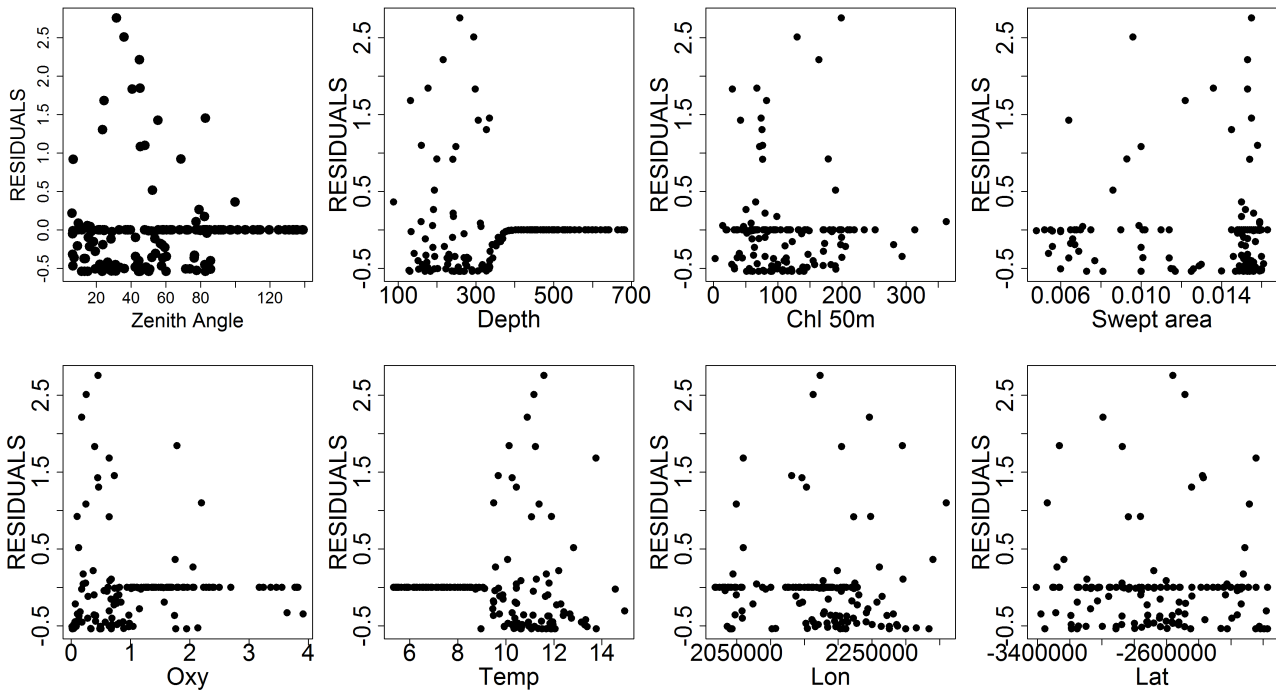
Figure S1: Pearson residuals plotted against all covariates for the Negative binomial GAM applied to the catch rates of M. capensis of all four size groups.
