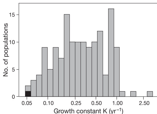
Fig. 4. Distribution of growth constant K of the von Bertalanffy growth function (VBGF) of 147 different bivalve populations from all over the world. Data are from a databank started by Brey (1999). Logarithmic scale on x-axis. Black bar: Arctica islandica , grey bars: others
