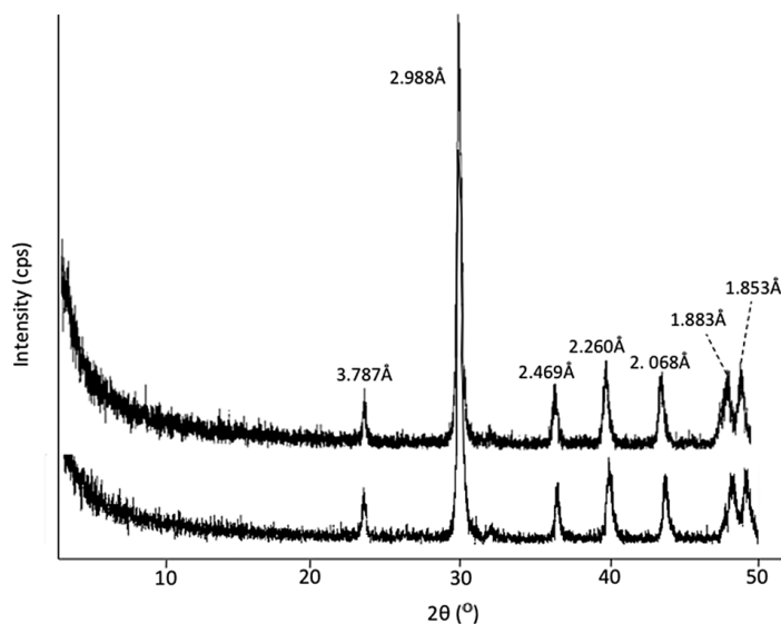
Fig. 2. Living (top) and non-living (bottom) maerl X-ray diffractograms. Peak d -spacings are labelled (Å)
