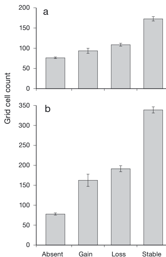
Fig. 5. BIOMOD consensus model projected absent, gain, loss and stable summary count matched to the (a) mean elevation and (b) elevation range of the 10 × 10 km grid cells. Vertical bars: ± SE
