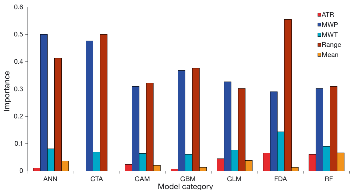
Fig. 3. Relative importance of the variables used to model the active blanket bog distribution. Variable importance was calculated as 1 minus the correlation between standard prediction and the prediction where the considered variable was randomised. ATR: annual temperature range, MWP/MWT: mean winter precipitation/temperature, Range: elevation range, Mean: mean elevation. See Table 1 for model acronyms
