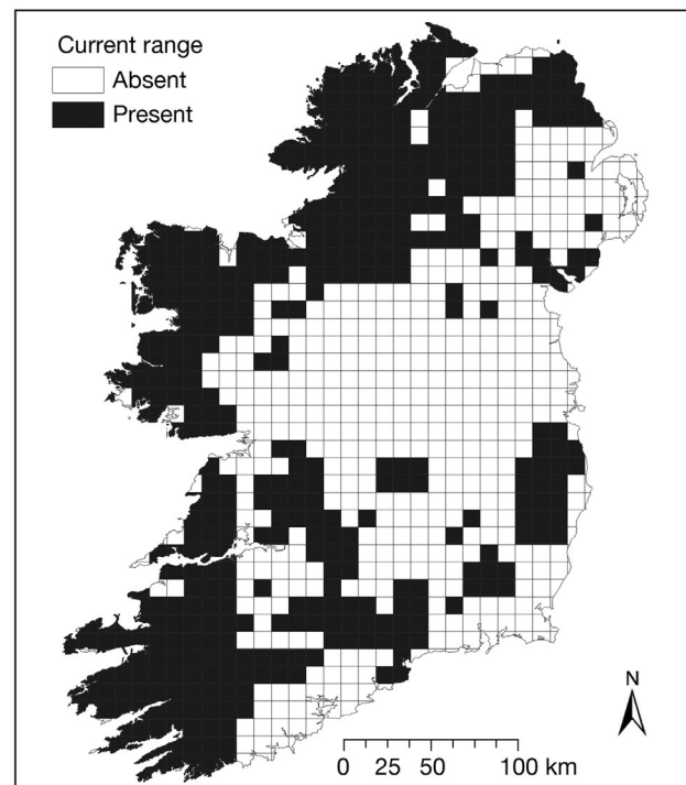
Fig. 1. Current distribution of active blanket bog in Ireland based on National Parks and Wildlife Service data (Ireland) and Joint Nature Conservancy Council data (Northern Ireland). Squares: habitat presence (black) or absence (white)
