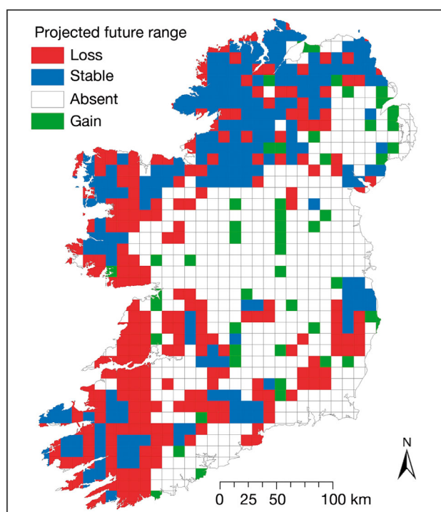
Fig. 4. Mapped BIOMOD consensus model output for the active blanket bog habitat based on a principal components analysis (PCA) of the median probability values and the true skill statistic (TSS) threshold. Red squares: projected losses of climate space for the A1B 2031–2060 scenario relative to the baseline; blue squares: stable climate space grids; green squares: potential climate space gains relative to the baseline
