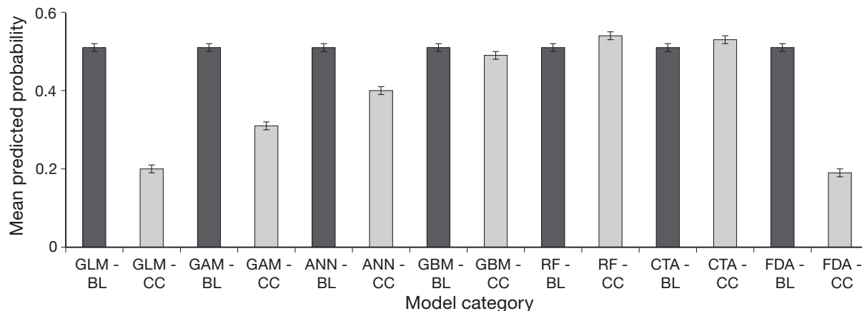
Fig. 2. Summary comparison of the predictive performance of the 7 models implemented in BIOMOD illustrating the mean probability distribution shifts associated with the climate change projections (CC; 2031–2060) compared to the baseline (BL; 1961–1990). Vertical bars: \pm SE. See Table 1 for model acronyms
