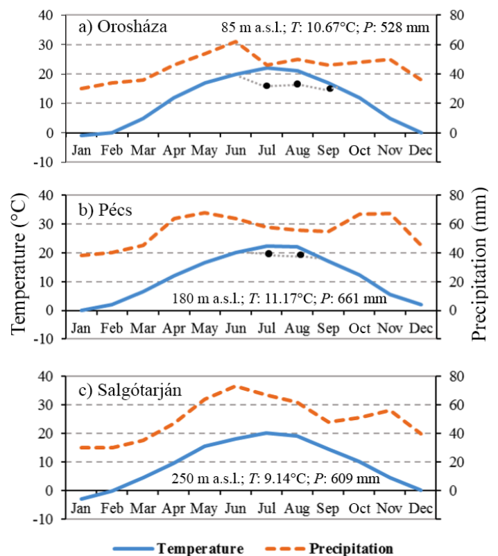
Fig. 3. Walter-Lieth climate diagrams of (A) Orosháza ( 46^{\circ} 34' \text{N} , 20^{\circ} 41' \text{E} ), (B) Pécs ( 46^{\circ} 00' \text{N} , 18^{\circ} 14' \text{E} ) and Salgótarján ( 48^{\circ} 06' \text{N} , 19^{\circ} 38' \text{E} ) meteorological stations (see Fig. 1). Points below the temperature diagram are the cut-off points of the semi-aridity curve ( 2/3 \times precipitation line). a.s.l.: above sea level; T: mean temperature; P: mean precipitation
