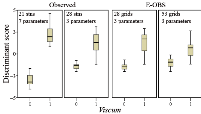
Fig. 5. Summary of the results from the 4 discriminant analyses on climatic factors that are related to the presence (1) or absence (0) of Viscum album album . The first 2 diagrams are based on meteorological data from meteorological stations from the period 1900–1950. The second 2 diagrams are based on recent E-OBS grids data from the period 1950–2010. The scores on the leftmost diagram are based on the discriminant function involving 7 independent variables (mean July temperature, air temperature sum of the vegetation period, average annual extreme minimum temperature, average annual extreme maximum temperature, the Gausson–Bagnouls aridity index calculated for July, annual fluctuation of mean temperature and relative humidity at 14:00 h in July). In the other 3 cases, the discriminant function involves 3 variables (mean July temperature, air temperature sum of the vegetation period and Gausson–Bagnouls aridity index calculated for July)
