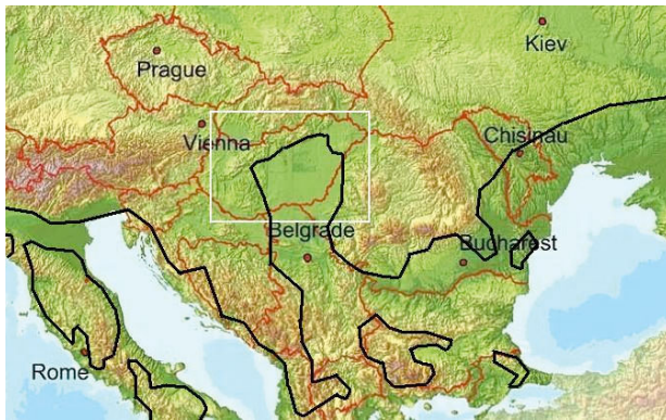
Fig. 2. The SE European section of the distribution of Viscum album album . After Jalas & Suominen (1976) and Kahle-Zuber (2008), modified after Săvulescu (1952), Flora Croatica Database ( http://hirc.botanic.hr/fcd/ ) and our own data. The white square indicates the area of the local map shown in Fig. 1; the bold black line marks the simplified (southern and isolated) boundary of the subspecies
