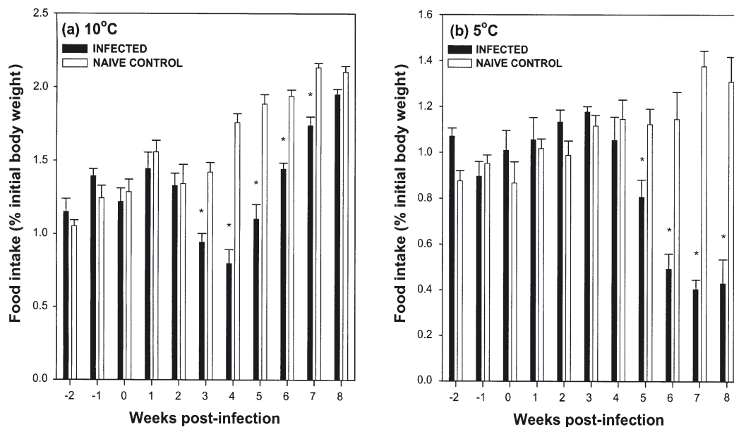
Fig. 1. Oncorhynchus mykiss infected with Cryptobia salmositica . Food intake (weekly mean \pm SE; % of initial body weight) by juveniles ( n = 13 group ^{-1} dose of 20 000 parasites fish ^{-1} ) and naïve controls at (a) 10°C and (b) 5°C. *Significantly lower than naïve controls
