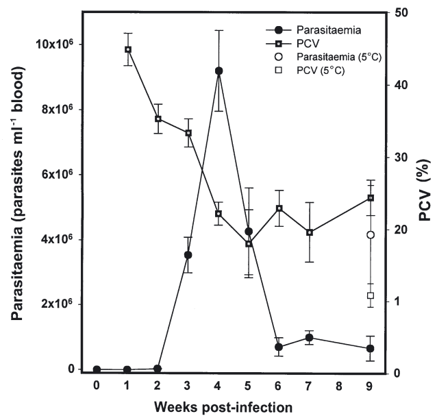
Fig. 2. Oncorhynchus mykiss infected with Cryptobia salmositica . Parasitemia and pack cell volume (PCV) values (mean \pm SE) of juveniles ( n = 5 per sample) infected with 20000 C. salmositica over the course of infection at 10°C (solid symbols); open symbols: values at 5°C at 9 wk post-infection
