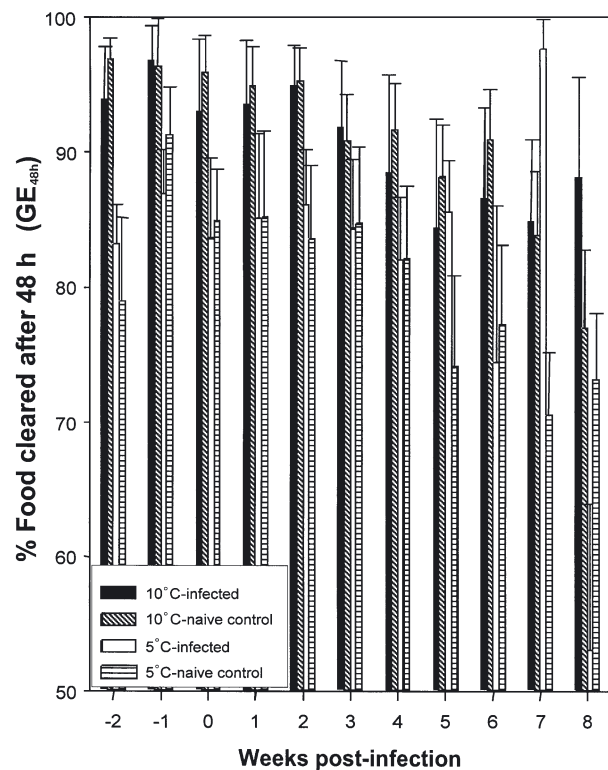
Fig. 3. Oncorhynchus mykiss infected with Cryptobia salmositica . Food cleared (mean percentage \pm SE) by juveniles at 10 and 5°C after 48 h ( n = 13 group ^{-1} )
