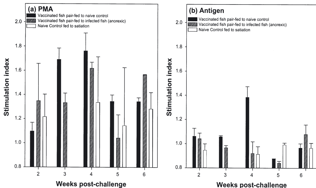
Fig. 4. Stimulation index (mean \pm SE) of macrophages stimulated with (a) PMA and (b) Cryptobia salmositica lysate from fish that were vaccinated with a live C. salmositica vaccine
