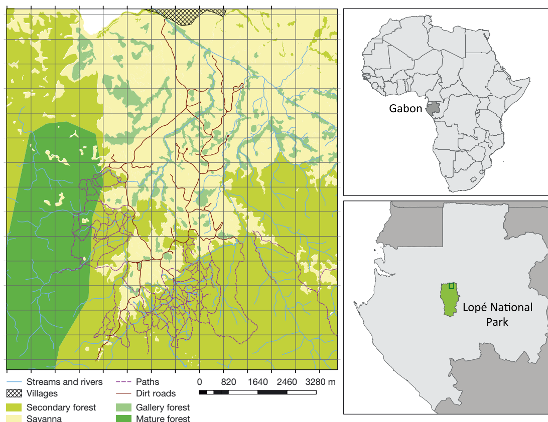
Fig. 1. Station d'Etudes des Gorilles et Chimpanzees (SEGC) study zone (left) from Schuttler et al. (2014). The green rectangle in Lopé National Park (LNP) represents the SEGC study zone area (bottom right)
