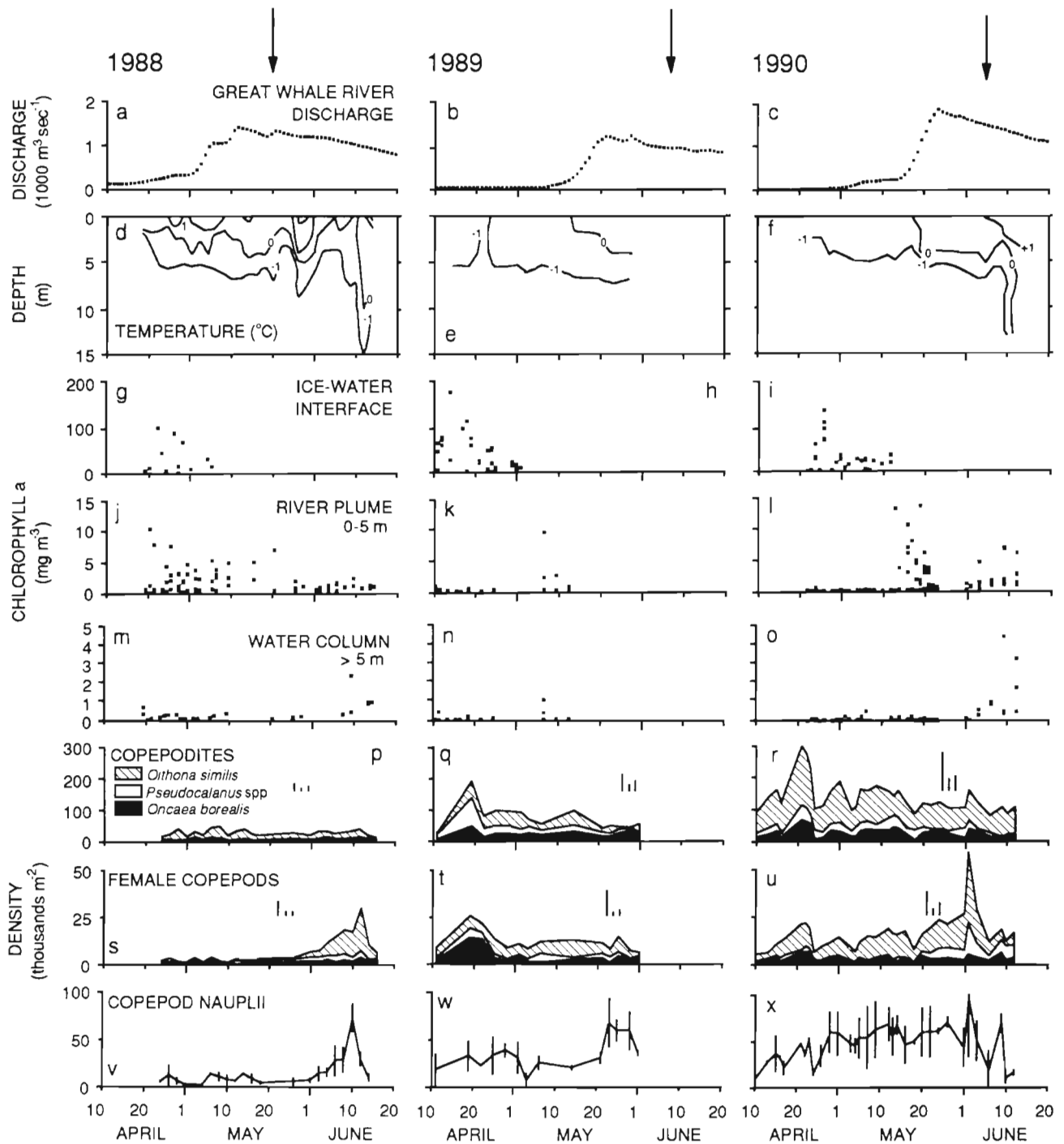
Fig. 2. Southeastern Hudson Bay in spring. Interannual comparison of (a to c) the timing of the Great Whale River freshet, (d to f) the temperature regime under the ice cover at station B, (g to i) the biomass of ice algae and (j to l) phytoplankton in the river plume and (m to o) in the water column, (p to r) the areal density of copepodites, (s to u) female copepods and (v to x) copepod nauplii ( \pm 1 standard deviation). All values of microalgal biomass available for each station were plotted. Zooplankton densities are averages of 4 (1988), 2 (1989) or 3 (1990) stations. The 3 vertical bars associated with copepodite and female copepod densities (p to u) correspond to 2 average standard deviations in the density of Oithona similis , Pseudocalanus spp. and Oncaea borealis from left to right respectively, and represent between-station variability. Vertical arrows indicate the beginning of the ice break-up in Hudson Bay
