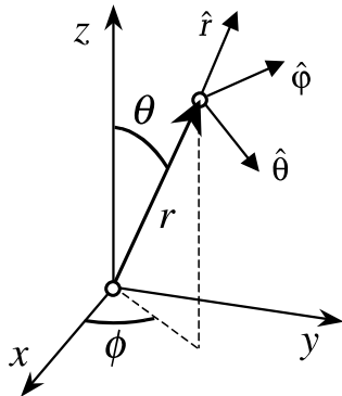
Fig. 2. Spherical polar co-ordinates (r, \theta, \phi) in relationship to Cartesian coordinates (x, y, z) . Unit vectors \hat{r} , \hat{\theta} and \hat{\phi} point in r , \theta and \phi directions respectively
