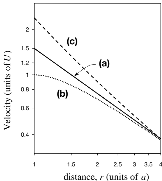
Fig. 10. Three models for feeding current structure (velocity scale U and effective radius a ). The pure stokeslet (a) has a r^{-1} dependence, the spherical pump (b) approaches a flatter - spatial dependence close to source, and the stokeslet + stresslet model (c) has a steeper dependence close to the source
