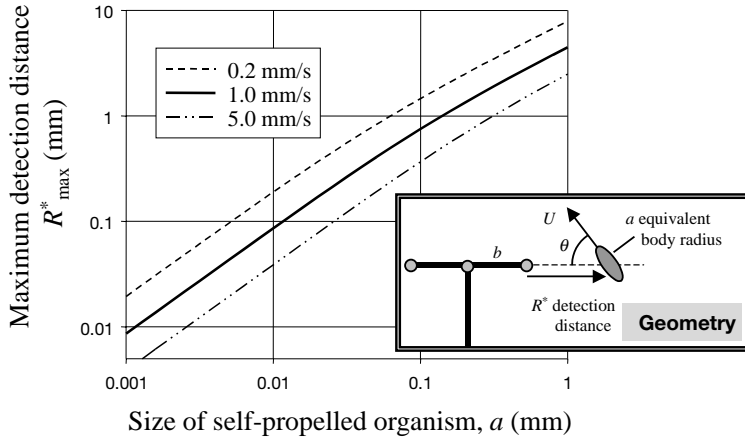
Fig. 8. Maximum detection distance R^*_{\max} , as a function of the equivalent spherical radius of a self-propelled organism. Curves are plotted for 3 different translational velocities, U = 0.2, 1 and 5 \text{ mm s}^{-1} . The sensitivity s = 40 \mu\text{m s}^{-1} and antenna length b = 1 \text{ mm} . The curves are for the particular detector-translation alignment shown in inset. Actual detection distance R^* depends on the angle of approach, \theta : R^* = \frac{1}{2}R^*_{\max}|3\cos^2\theta - 1|
