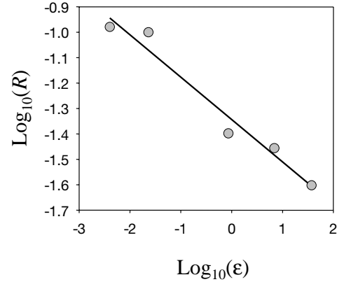
Fig. 18. Acartia tonsa . Estimated reaction distance, R (cm), as a function of dissipation rate, \epsilon ( \text{cm}^2 \text{s}^{-3} ), for the copepod feeding on the ciliate Strombidium sulcatum in a laboratory study (Kjørboe & Saiz 1995). Reaction distance estimated from observed clearance rates, \beta_o and by numerically solving the encounter equation \beta_o = \pi R^2 (U^2 + 2\alpha^2 (\epsilon R)^{2/3})^{1/2} . The Kolmogorov scale ranges from about 1 mm to 100 \mu\text{m} , which is \leq the length scale of A. tonsa (antenna span, 2b = 2 mm)
