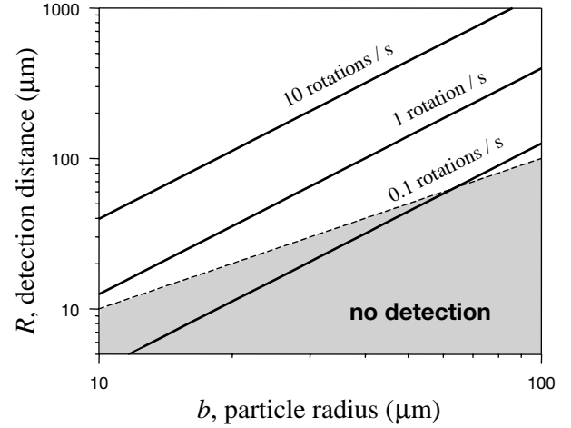
Fig. 13. Detection distance, R , of a rotating organism of radial dimension b . In this example, we assume that the detector is large compared to b , and detection is triggered when the velocity exceeds 40 \mu\text{m s}^{-1} . The no detection zone is defined as when R < b . Three detection curves are plotted, for rotation rates of 0.1, 1 and 10 rotations \text{s}^{-1} .
