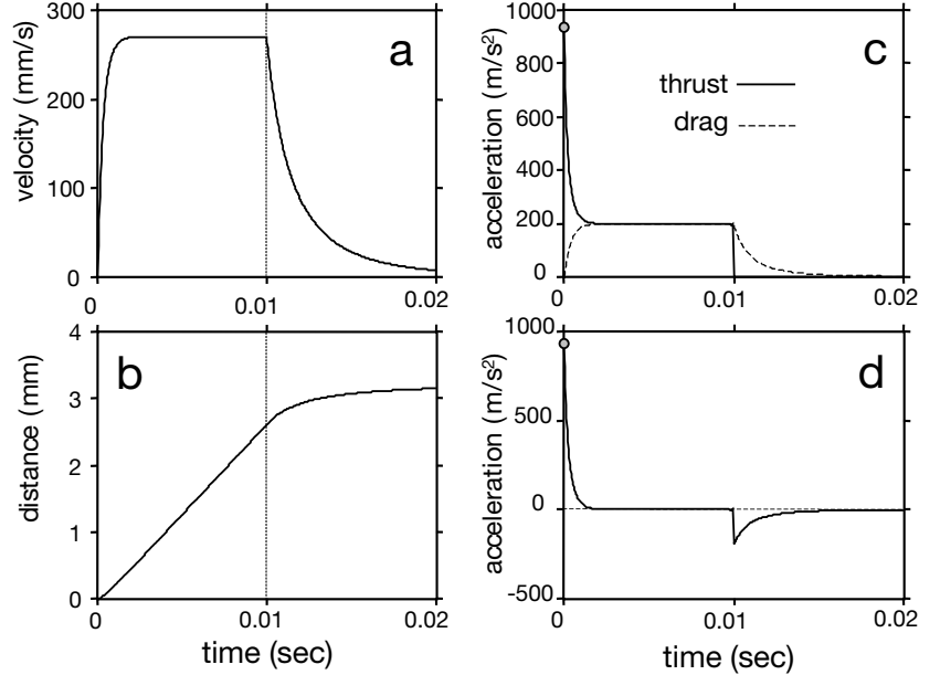
Fig. 16. Simulation of the power stroke of a copepod escape jump. The copepod has an effective radius of 0.2 mm, and a maximum 'pumping' velocity of 500 \text{mm s}^{-1} . Thrust is applied for 10 ms. (a) Velocity; (b) distance (c) and (d) acceleration (force per unit mass) experienced by the copepod (thrust and drag) and by the fluid respectively
