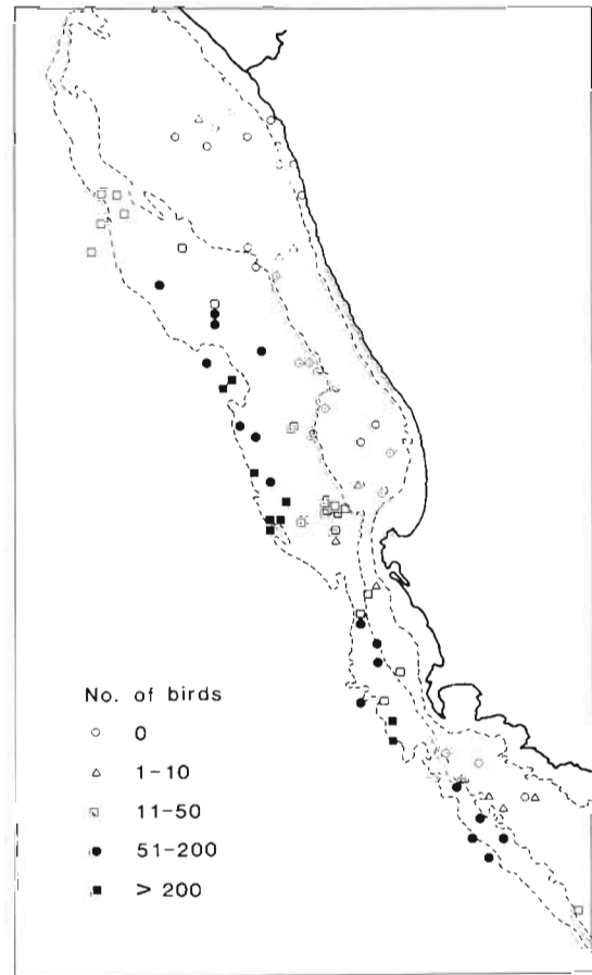
Fig. 4. Numbers of black-browed albatrosses attending trawls
