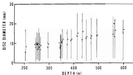
Fig. 7. Ophiura sarsii . Relationship between size structures and depth in the area off Ōtsuchi. (○) Mean values of size; vertical bars: ranges (minimum and maximum values) of size; (◄) mode of large individuals. Mean size, maximum size and mode of adults increased with depth
