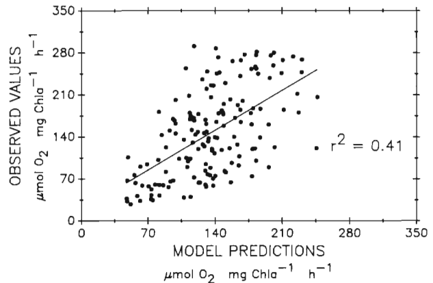
Fig. 3. Observed vs predicted plot for the curvilinear regression model. Equation and constants are given in Table 3
