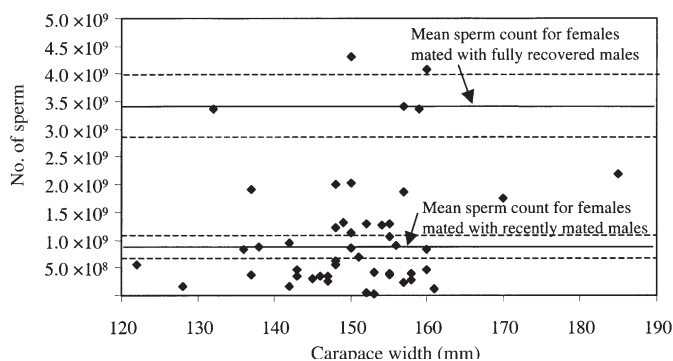
Fig. 2. Callinectes sapidus . Carapace width and sperm counts of ejaculate for mature females sampled from Rhode River ( n = 47 ). Upper and lower sets of solid and dashed lines: mean sperm count and standard error of the mean for females in laboratory experiments receiving sperm from fully recovered and recently mated males respectively
