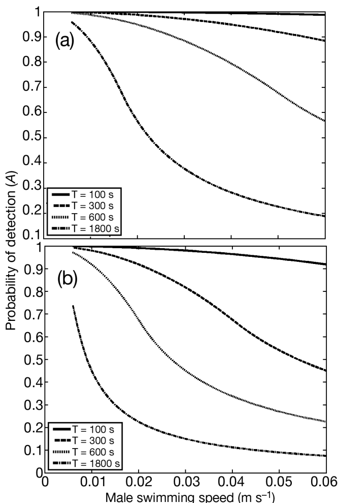
Fig. 1. Probability (A) of the male detecting a female while crossing her detection zone, as a function of male swimming speed v (m s -1 ) and the period, in seconds, of the female's flashing ( T ); calculated using Eqs. (4), (5) & (6). In (a) E = 10^{10} photons; in (b) E = 10^9 photons. Other parameter values: N = 5 ; \alpha = 0.05 m -1 ; D = 0.002 m
