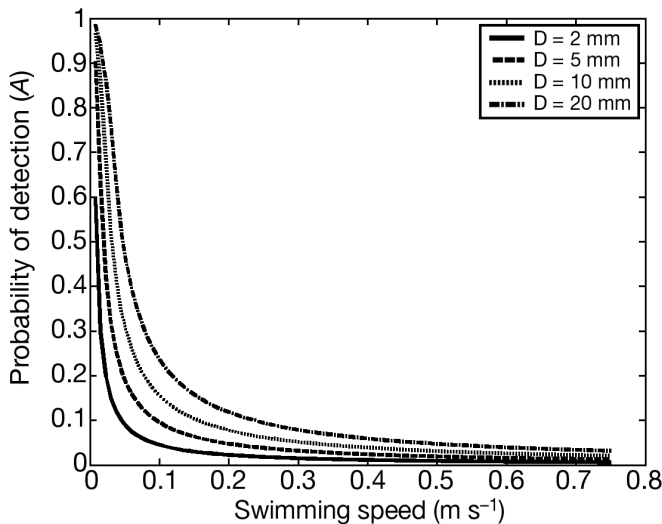
Fig. 2. Probability ( A ) of a fish (either a male conspecific or a predator) detecting the female while crossing her detection zone, as a function of swimming speed v ( m s^{-1} ) and pupil diameter D (in mm); calculated using Eqs. (4), (5) & (6). Other parameter values: N = 5 ; E = 10^{10} ; \alpha = 0.05 m^{-1} ; T = 1800 s
