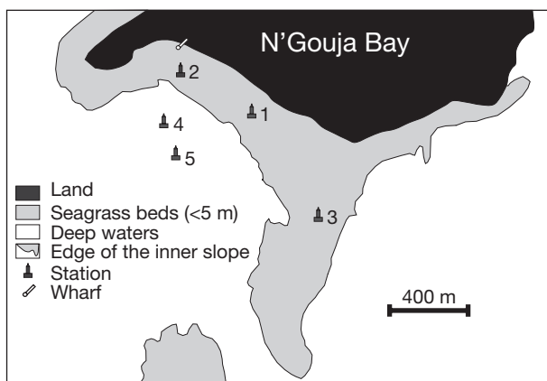
Fig. 1. Map of N'Gouja Bay, Mayotte, with the positions of the listening stations (▲). Stns 1 to 3 are within the seagrass bed; Stns 4 and 5 are positioned offshore. Wharf near Stn 2 indicates location on the beach where turtles were tagged
