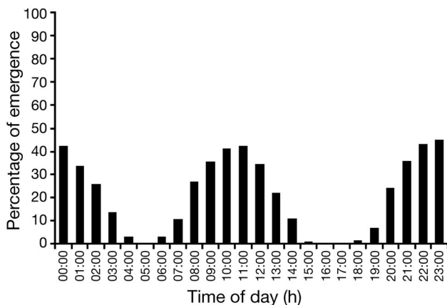
Fig. 3. Estimated percentage of the total time that listening Stns 1, 2 and 3 on the seagrass bed were emerged (due to low tides) for each hour of the day over the 31 d period from June 14 to July 14, 2003
