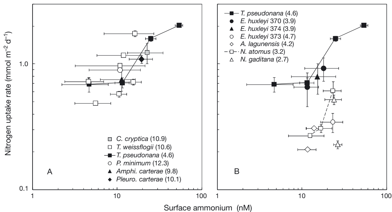
Fig. 5. Relationships between the absolute cellular nitrogen uptake rate (normalized to cell surface area) and \text{NH}_4^+ concentration at the cell surface computed from Eqs. (4) & (5). The CCMP clone numbers are given for the 3 Emiliana huxleyi strains. Data for Thalassiosira pseudonana are plotted in both panels for comparison. For full species names see Table 1. Error bars: \pm SD
