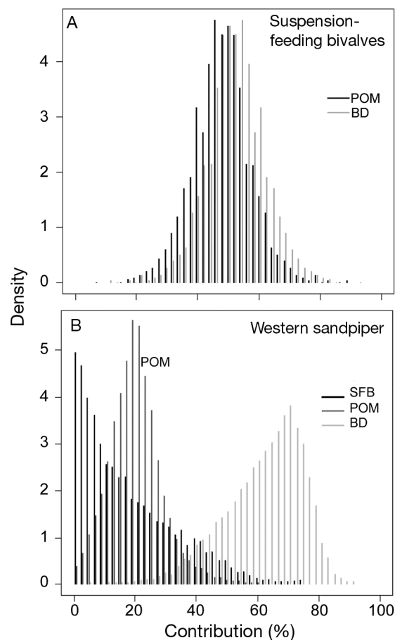
Fig. 3. Probability distributions of contributions of potential food sources in diets of (A) suspension-feeding bivalves (SFB) and (B) western sandpiper at Roberts Bank stopover obtained using the SIAR mixing model. BD: benthic diatoms; POM: particulate organic matter. The highest probability contributions for the SFB diet are 50% POM and 50% BD, whereas the highest probability contributions for the western sandpiper diet were >75% BD, 20% POM, and <5% SFB
