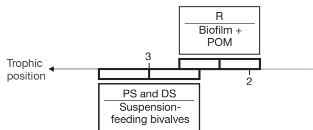
Fig. 4. Calidris mauri . Major components of western sandpiper diets and trophic positions at proximate and distal stopover grounds (PS and DS) prior to arrival at Roberts Bank stopover (R), as given by the \delta^{13}\text{C} and \delta^{15}\text{N} of muscle (DS), liver (PS), and stomach contents (R). Bold rectangles represent SD of the means
