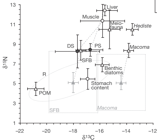
Fig. 2. \delta^{13}\text{C} and \delta^{15}\text{N} (‰) of potential food sources ( \Delta ) and western sandpiper compartments ( \circ ). Means \pm SD. Dietary isotopic values ( \bullet ) were obtained by subtracting trophic enrichment (dashed lines) of 1.9 and 3.1 ‰ for muscle, and 1.1 and 4 ‰ for liver (Evans-Ogden et al. 2004) from carbon and nitrogen deviations, respectively. The ellipse groups together the sources at Roberts Bank stopover which contributed to diet. The \Delta and rectangles represent the ranges of possible diet isotopic deviations of suspension-feeding bivalves (SFB: Mya sp. and Tapes philippinarum ) and Macoma sp., taking into account the range of published fractionation values (−0.90 to 2.04 and 1.14 to 5.40 ‰ for carbon and nitrogen, respectively; Post 2002, Yokoyama et al. 2005, 2008, Dubois et al. 2007). Only isotopic composition of liver vs. muscle was not statistically significant (ANOVA, p > 0.05 ). POM: particulate organic matter; R: Roberts Bank stopover; PS: proximate stopovers; DS: distal stopovers
