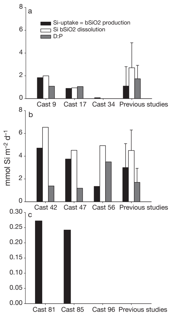
Fig. 5. Integrated (100 to 1% photosynthetically active radiation) Si(OH) 4 uptake (i.e. bSiO 2 production) and bSiO 2 dissolution rates, and dissolution:production ratios (D:P). Panels a, b, and c represent P1 (western SAZ), P2 (PFZ), and P3 (eastern SAZ), respectively. Previous studies show the summer values of earlier studies for each area (Caubert 1998, Brzezinski et al. 2001, Quéguiner 2001, Leblanc et al. 2002, Beucher et al. 2004). PFZ: Polar Frontal Zone; SAZ: Subantarctic Zone. Values for Cast 96 were below detection limit, and no previous studies are available for the eastern SAZ (Panel C)
