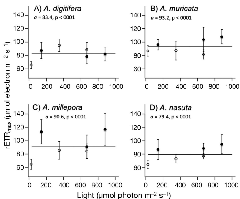
Fig. 7. Relative maximum electron transfer rates ( rETR_{max} ) for (A) Acropora digitifera , (B) A. muricata , (C) A. millepora and (D) A. nasuta versus light intensity for corals deployed in the field (●) and in the laboratory (○). Lines: linear regression fitted to all the data ( y = a ). Data points are average of 151 samples with error bars (SE). Fitted coefficient of linear regression ( y = a ), and the statistical significance of its difference from zero are shown
