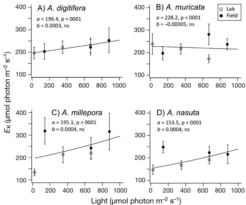
Fig. 8. Subsaturating irradiance ( E_K ) for (A) Acropora digitifera , (B) A. muricata , (C) A. millepora and (D) A. nasuta versus light intensity for corals deployed in the field (●) and in the laboratory (○). Lines: non-linear regression (exponential) fitted to all the data. Data points: mean of 144 samples with error bars (SE). Fitted coefficients of non-linear regression ( y = a \times e^{bx} ) and the statistical significance of their difference from zero are shown
