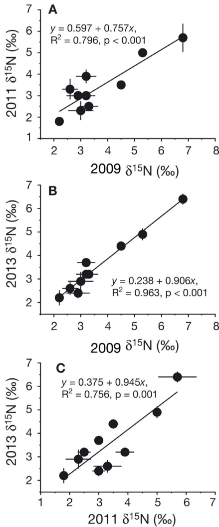
Fig. 5. Relationship between \delta^{15}\text{N} values of seagrasses (mean \pm SE) from year to year. Each point represents one of 10 sites monitored in 2009, 2011, and 2013
