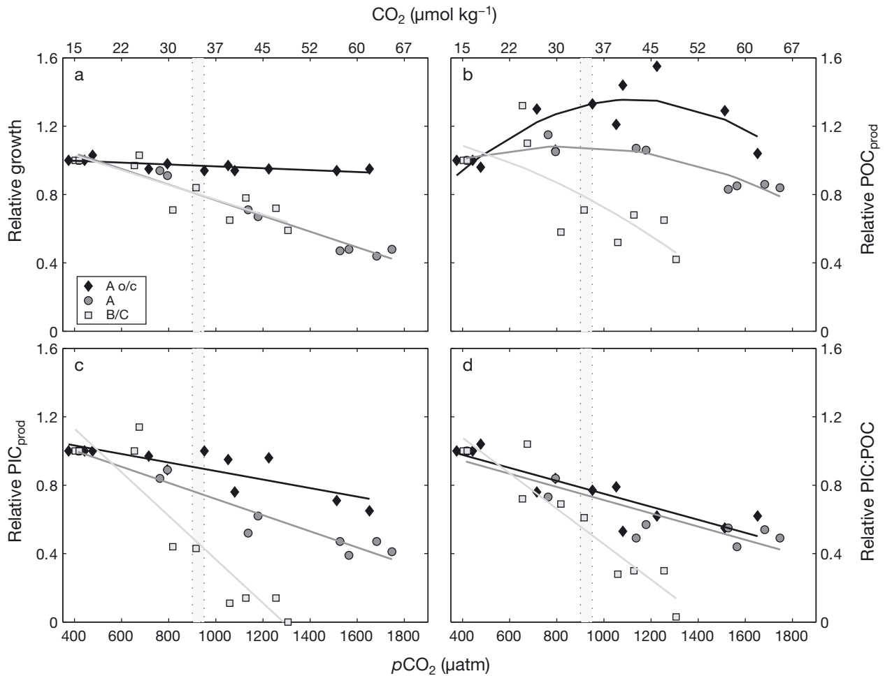
Fig. 4. Relative change in (a) growth, production rate of (b) particulate organic carbon ( \text{POC}_{\text{prod}} ) and (c) particulate inorganic carbon ( \text{PIC}_{\text{prod}} ), and (d) PIC:POC ratio in response to p\text{CO}_2 and \text{CO}_2 . Gray shaded areas correspond to the projected p\text{CO}_2 values for the end of this century in the Southern Ocean according to Intergovernmental Panel on Climate Change (IPCC) scenario RCP8.5. Solid lines represent the best fit using Matlab tool 'polyfit'
