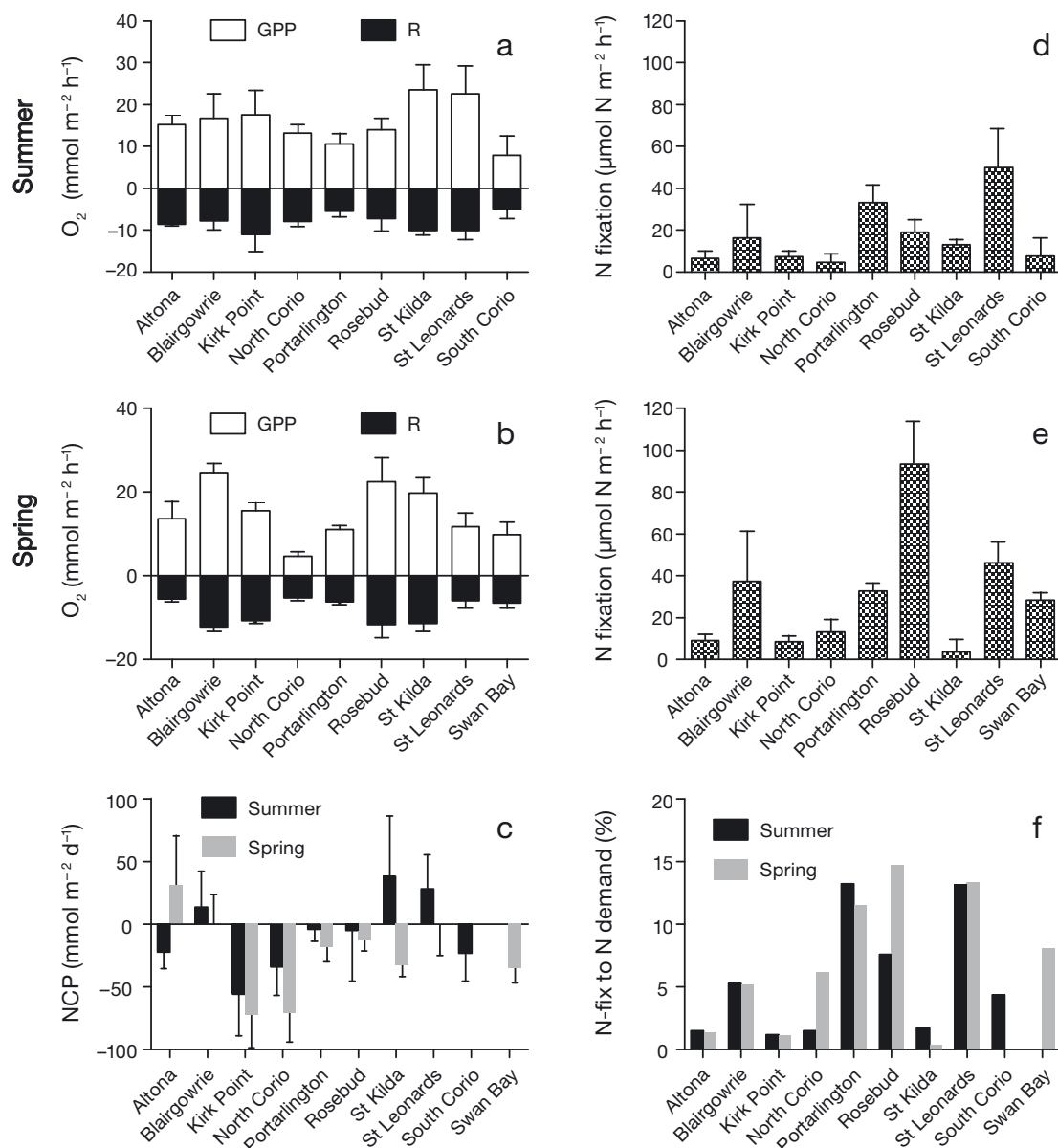
Fig. 2. Rates of gross primary production (GPP) and respiration (R) during (a) summer and (b) spring. (c) Rates of daily net community production (NCP) during both seasons. Nitrogen fixation during (d) summer and (e) spring (mean \pm SD, n = 4 ). (f) Rate of nitrogen fixation as a percent of total estimated nitrogen demand by Zostera spp. (see 'Materials and methods' for calculation)
