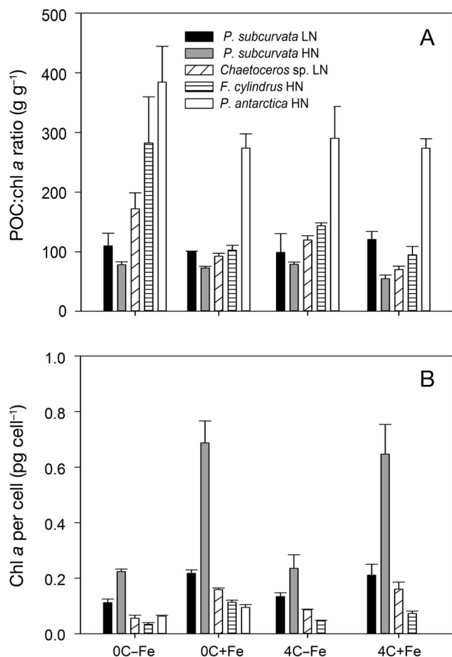
Fig. 5. (A) Particulate organic carbon (POC) to chl a ratio ( \text{g g}^{-1} ) and (B) chl a per cell ( \text{pg cell}^{-1} ) of Pseudo-nitzschia subcurvata , Chaetoceros sp., Fragilariopsis cylindrus , and Phaeocystis antarctica cultures grown in either in high (HN) or low (LN) nutrient levels, at either 0 or 4°C, under iron-limited (-Fe) or iron-replete (+Fe) conditions
