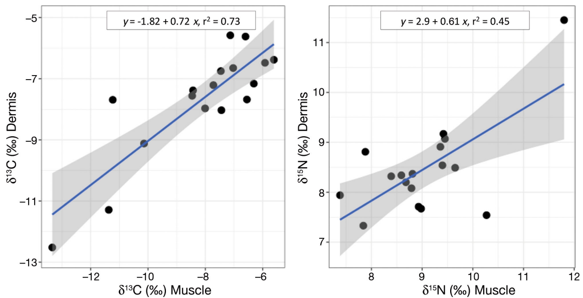
Fig. 2. Linear regressions for stable isotope values generated from chemically extracted dermis and muscle tissue for nurse sharks Ginglymostoma cirratum ( n = 17 ). Grey shaded area represents standard error, blue line represents line of best fit
