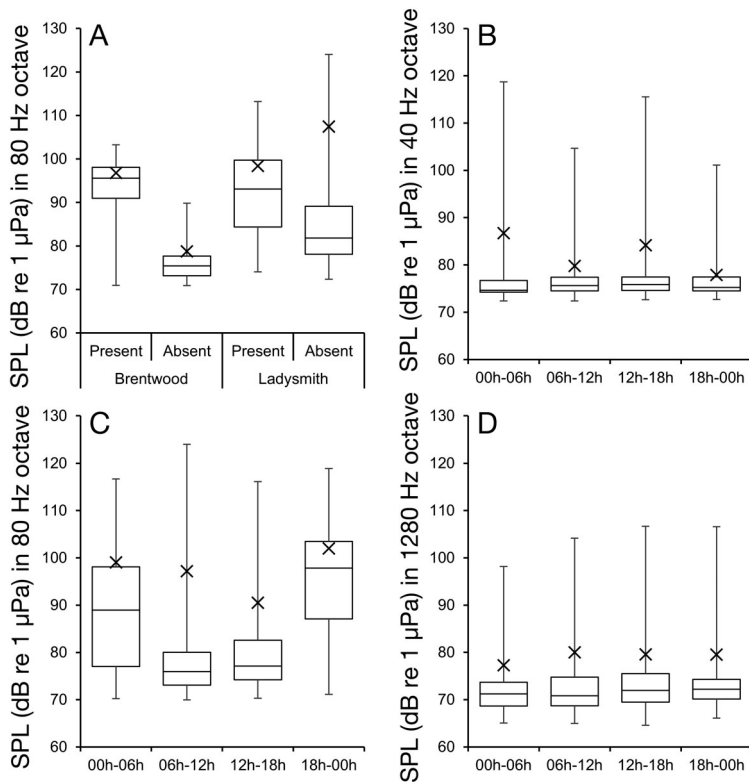
Fig. 6. Impact of the presence of plainfin midshipman Porichthys notatus hums at 2 deployment sites (Brentwood Bay and Ladysmith Inlet) on sound pressure levels (SPLs) in (A) the 80 Hz octave band, and trends in SPL in (B) 40, (C) 80, and (D) 1280 Hz octave bands throughout the deployments at Brentwood Bay and Ladysmith. Boxes: interquartile range; lines within the boxes: median values; whiskers: minimum and maximum values. × symbols: arithmetic means
