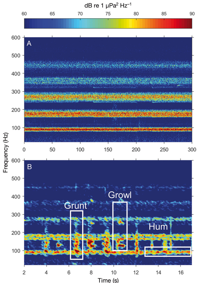
Fig. 1. Spectrograms of plainfin midshipman Porichthys notatus (A,B) hums and (B) hums, grunts and growls. Sample rate = 48 kHz. Fast Fourier transform (FFT) window size = 12 000 for (A) and 6000 for (B). Each spectrogram has a 50% overlap and uses a Hanning window
