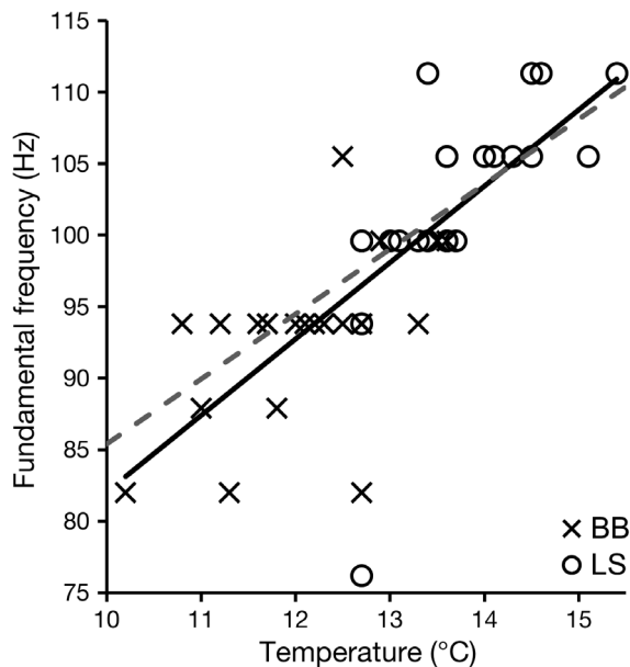
Fig. 3. Relationship between temperature and the fundamental frequency of the plainfin midshipman Porichthys notatus hum at Brentwood Bay (BB) and Ladysmith Inlet (LS) recorded near Vancouver Island, Canada. Solid black line: linear regression fit for the pooled data; grey dashed line: trend from Brantley & Bass (1994)
