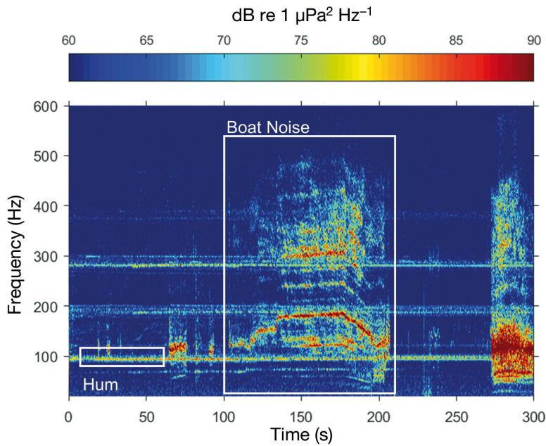
Fig. 5. Spectrogram of plainfin midshipman Porichthys notatus hum and boat noise present at the same time. Sample rate = 48 kHz. Fast Fourier transform (FFT) window size = 12 000. Each spectrogram has a 50% overlap and uses a Hanning window
