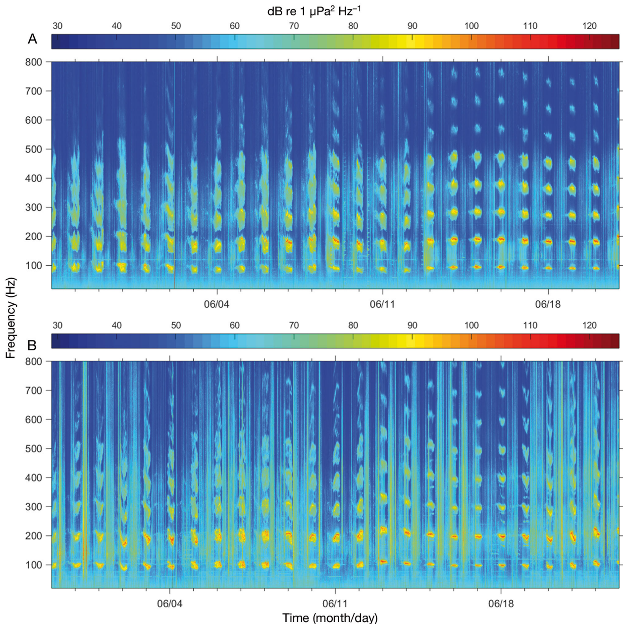
Fig. 2. Spectrogram for the full deployments at (A) Brentwood Bay and (B) Ladysmith Inlet, British Columbia, showing clear peaks in power spectral densities around 100 Hz every night throughout both deployments. The peaks are caused by the plainfin midshipman Porichthys notatus hum
