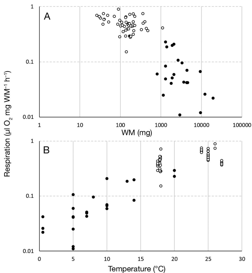
Fig. 1. Literature compilation of respiration rates (mass specific) of myctophid fishes versus (A) wet mass (WM) and (B) temperature. Note the logarithmic scales. (●) Data from direct oxygen consumption experiments; (○) respiration estimated from electron transport system (ETS) measurements
