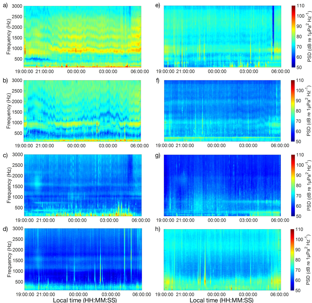
Fig. 4. Low-band (100–3000 Hz) power spectral densities (PSD) of recorded playbacks and original files used for playbacks for 2 representative nights; (a–d) 6–7 June 2016, for 3 playback treatments: (a) high, Site 4; (b) low, Site 2; (c) silent, Site 5, and (d) the original reef recording (not amplified) from Ram Head on 2–3 August 2013; (e–h) 20–21 July 2017, for 3 playback treatments: (e) high, Site 2; (f) low, Site 1; (g) silent, Site 3, and (h) the original reef recording (not amplified) from Tektite on 17–18 July 2017. PSD shown is integrated over 1 min time bins and in 1 Hz frequency bins. In (e), there was reduced PSD around 05:15:00 h for a 10 min period where the playback temporarily paused
