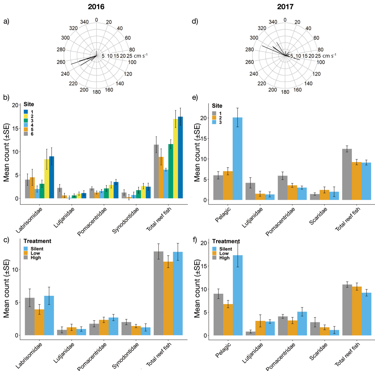
Fig. 5. Mean nightly current direction and magnitude for (a) 2016 and (d) 2017 with mean catch of common taxa by site in (b) 2016 and (e) 2017 and by intended acoustic treatment in (c) 2016 and (f) 2017
