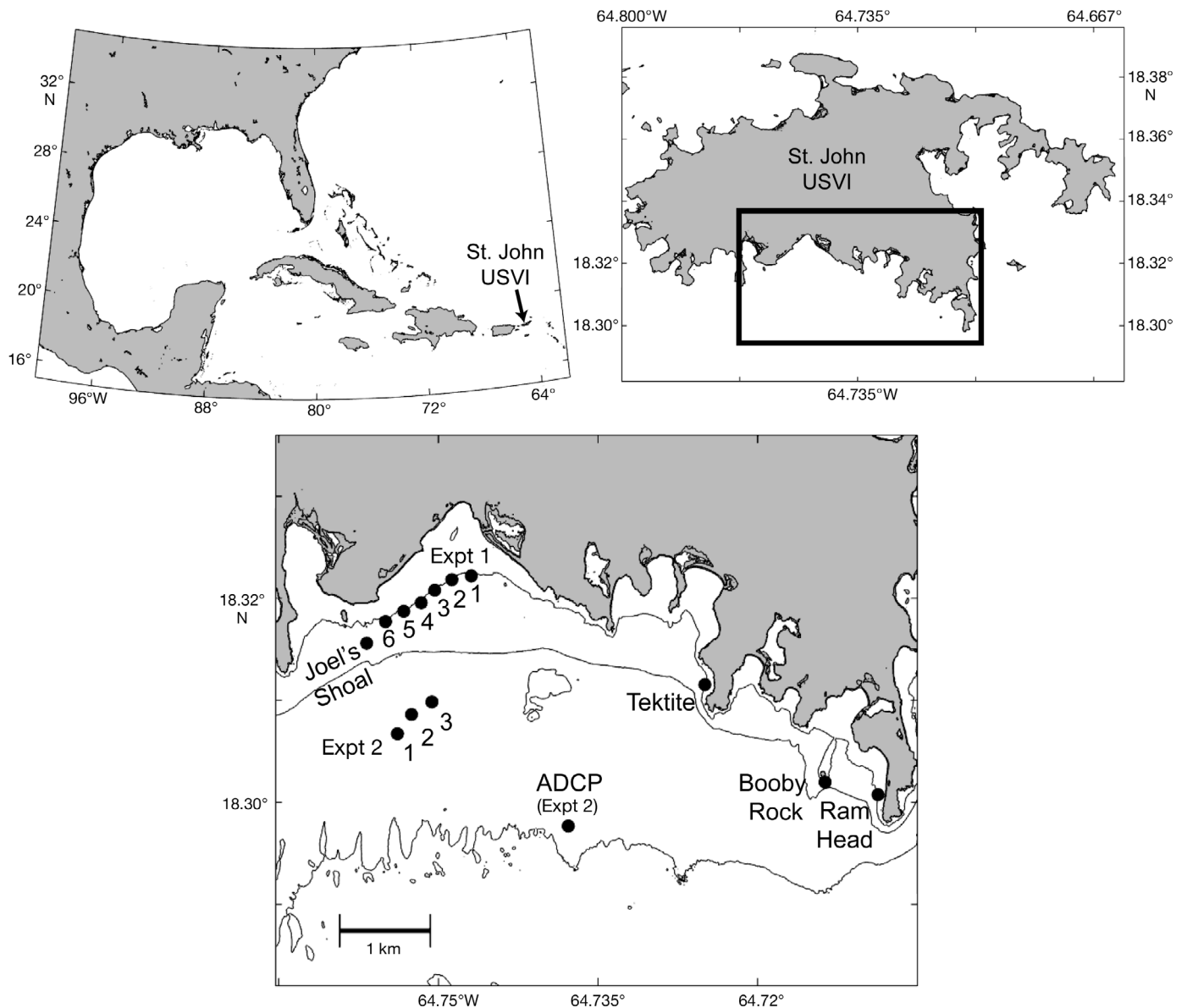
Fig. 1. Experiment locations on the south shore of St. John, including location of St. John within the greater Caribbean. Recordings from the reefs Tektite, Booby Rock, and Ram Head were used in playback experiments; Joel's Shoal represents the nearest reef to our experimental site. Thin lines: 10, 20, and 30 m isobaths
