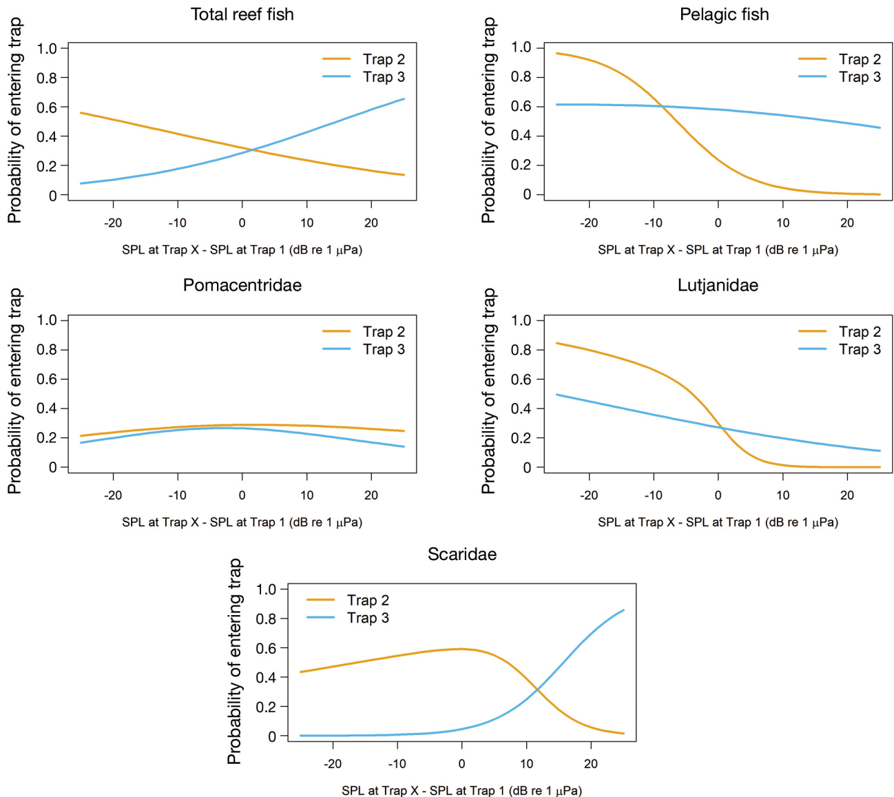
Fig. 7. Predicted probability curves indicating the change in probability of fish taxa entering a trap based on the difference in median low-band sound pressure level (SPL) between that trap and Trap 1. Gold lines: probability of entering Trap 2 based on a range of differences in median low-band SPL from Trap 1. Blue lines: probability of entering Trap 3 based on a range of differences in median low-band SPL from Trap 1
