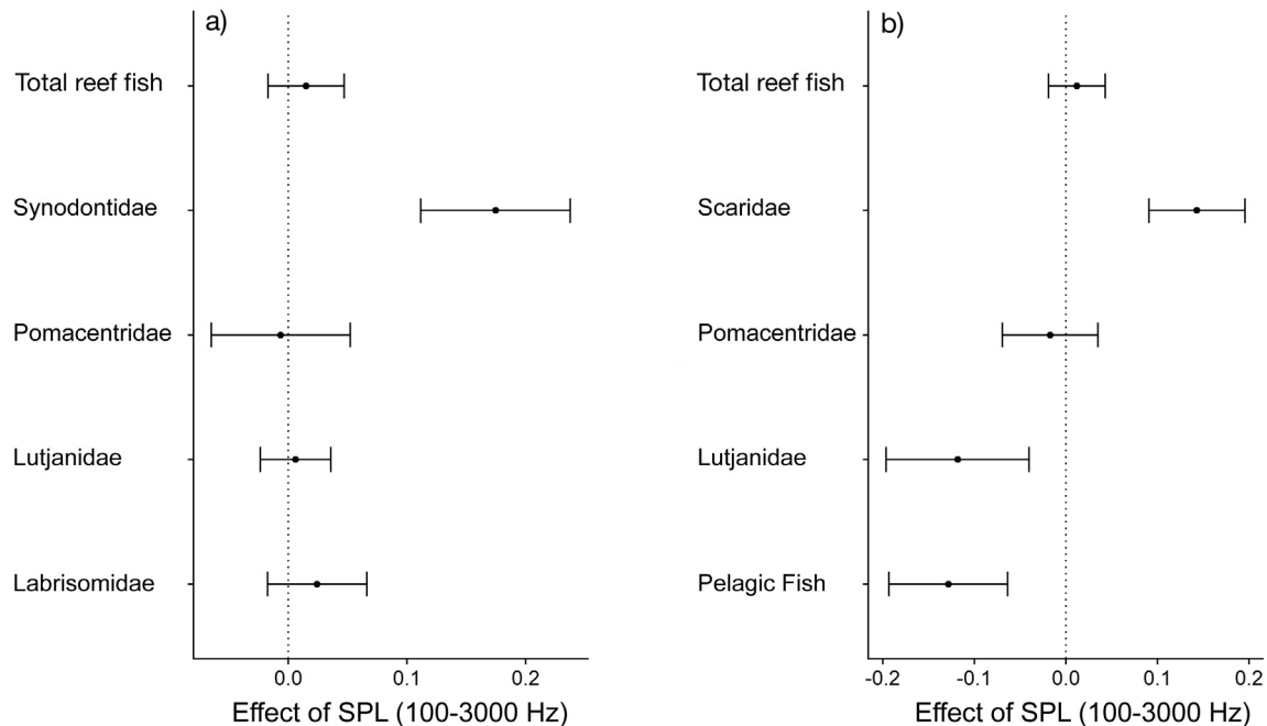
Fig. 6. Slope estimates ( \pm SE) of the effect of median low-band sound pressure level (SPL) on the catch of commonly caught larval fish taxa in (a) 2016 and (b) 2017
