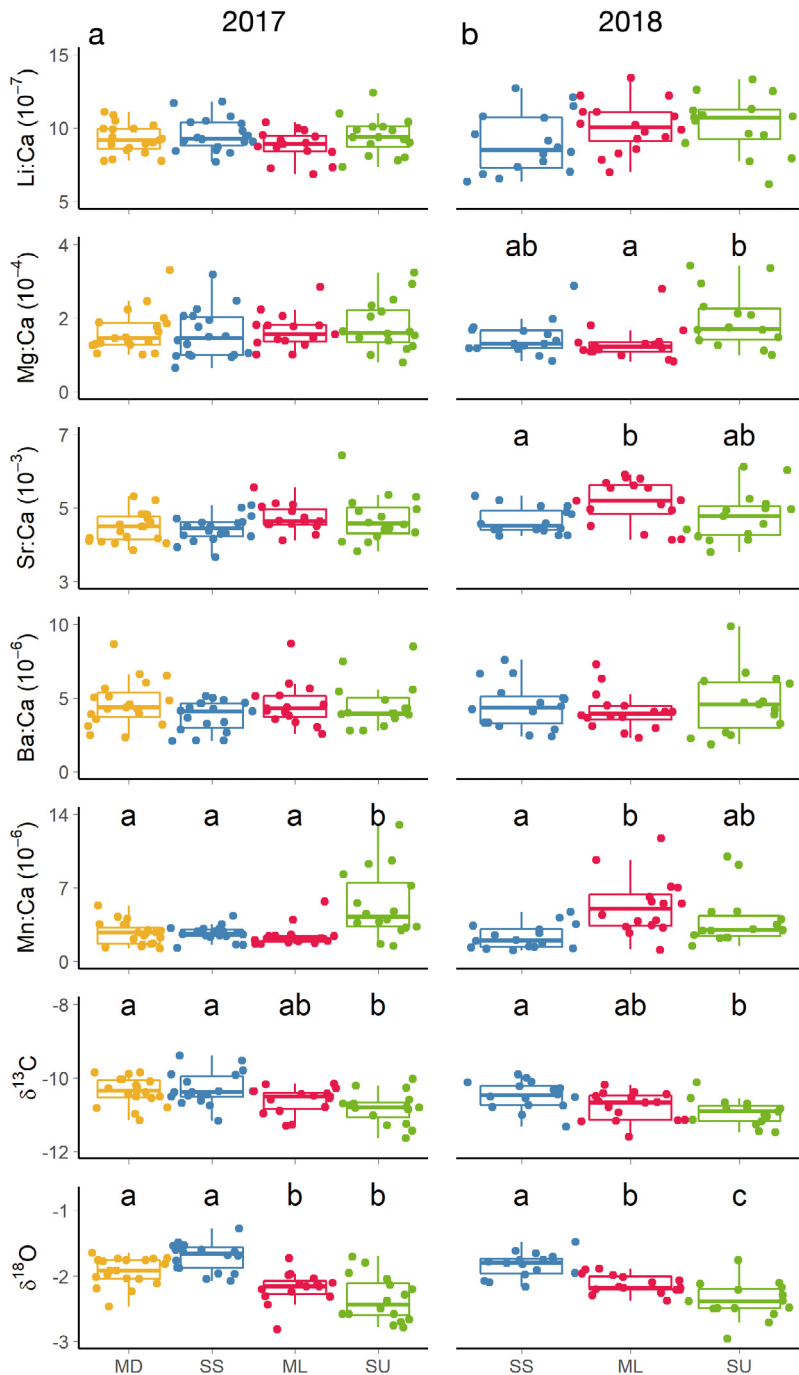
Fig. 5. Regional comparisons of otolith element:Ca ratios and stable isotope (‰) composition for young-of-the-year yellowfin tuna Thunnus albacares collected in 4 nursery areas in the Indian Ocean (MD: Madagascar; SS: Seychelles-Somalia; ML: Maldives; SU: Sumatra) for the 2017 and 2018 cohorts. Letters identify significant differences ( p < 0.05 ) between regions within a cohort. Interquartile range (25 th and 75 th percentiles) is shown by extent of boxes, and error bars represent the 10 th and 90 th percentiles. Median (50 th percentile) is also shown. Dots represent individuals
