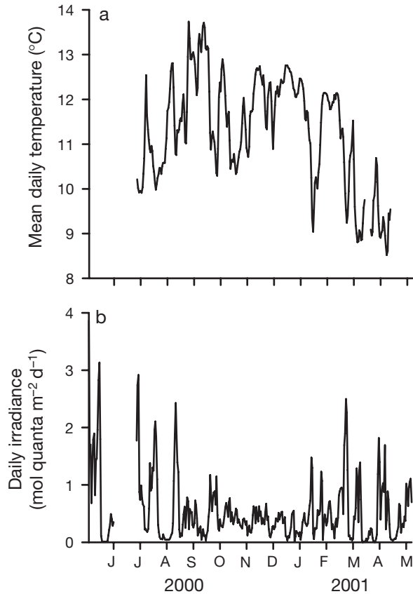
Fig. 2. Time series of (a) daily mean temperature and (b) total daily irradiance at the study site in Carmel Bay (depth = 30 m)
