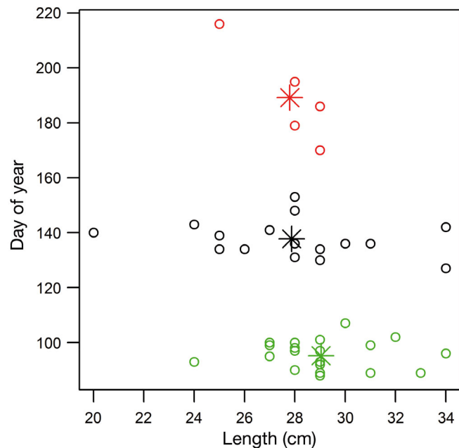
Fig. 3. Clustering analyses of the time of seaward departure by acoustically tagged Atlantic herring Clupea harengus ( N = 47 ) from the Landvik system vs. body size (total length, cm) between 29 March and 30 August 2012. The 3 groups were in part assigned to disparate population components: Landvik herring (red symbols), coastal Skagerrak spring spawning herring (green symbols) and Norwegian spring spawning herring (black symbols). Asterisks denote mean departure date for each clustered group
