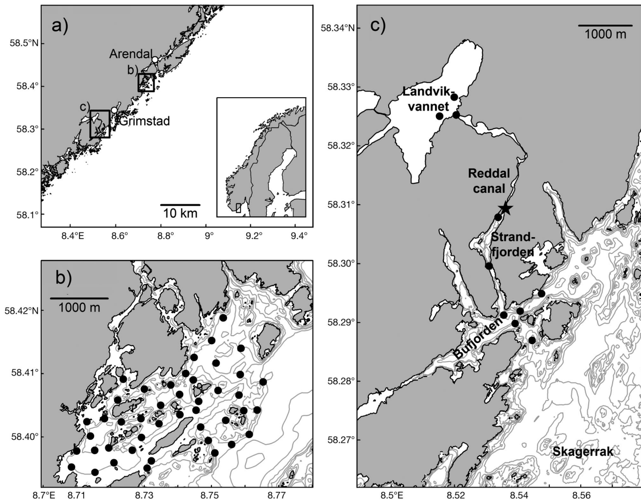
Fig. 1. (a) Study area along the Norwegian Skagerrak coast. (b) Location of the acoustic receiver array in Sömskilen near the town of Arendal. (c) Lake Landvikvannet and the connected fjords Strandfjorden and Bufjorden, showing the point of capture, acoustic tagging and release of Atlantic herring Clupea harengus (★), and positions of deployed acoustic receivers (●)
