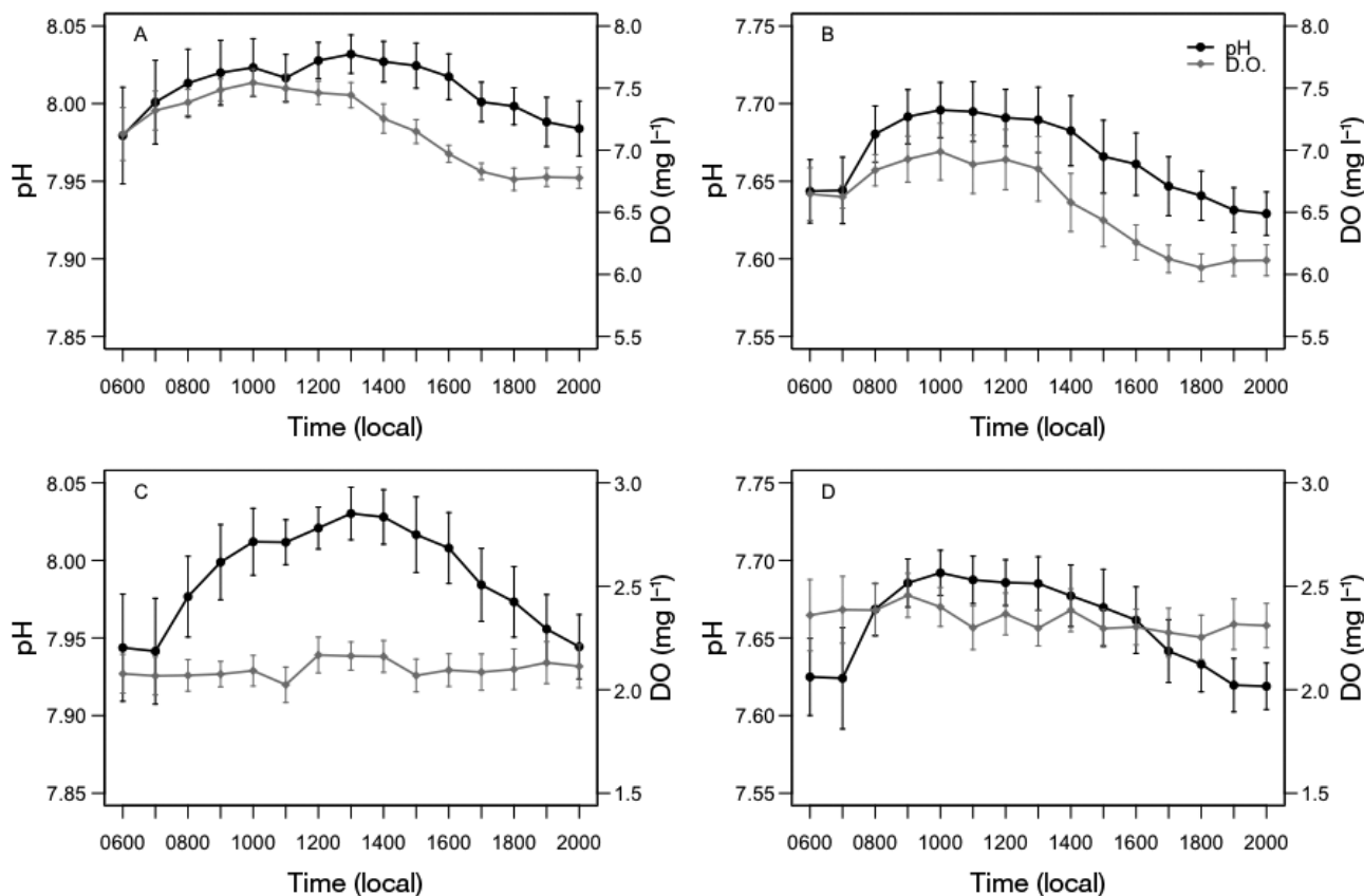
Fig. A1. Mean ( \pm SE) pH and DO measurements taken at hourly intervals throughout the day from 06:00 to 20:00 h local time in (A) control pH and dissolved oxygen (DO), (B) reduced pH and control DO, (C) control pH and low DO, and (D) reduced pH and low DO treatments
