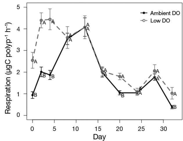
Fig. 2. Carbon-specific aerobic respiration rates ( \mu\text{gC polyp}^{-1} \text{h}^{-1} \pm SE) of Aurelia aurita polyps in the control dissolved oxygen (DO) treatments (solid black) and low DO treatments (dashed gray). Different letters (A, B) on a given day indicate significant differences ( p < 0.05 ) between groups; treatment details are given in Table 2
