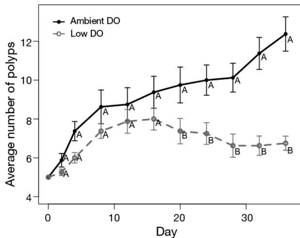
Fig. 1. Average number of Aurelia aurita polyps ( \pm SE) in the control dissolved oxygen (DO) treatments (solid black) and low DO treatments (dashed gray). Different letters (A,B) on a given day indicate significant differences ( p < 0.05 ) between groups; treatment details are given in Table 2
