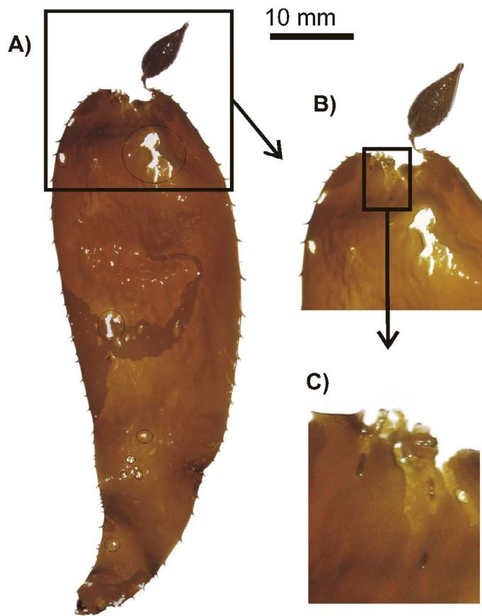
Fig. S2. Bircenna macayai . (a) Grazing marks, (b) close-up of grazing marks, and (c) close-up of feeding galleries
