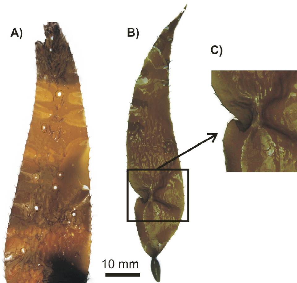
Fig. S1. Pseudopleonexes lessoniae . (a) Grazing marks, (b) blade with single nest, and (c) close-up of single nest
