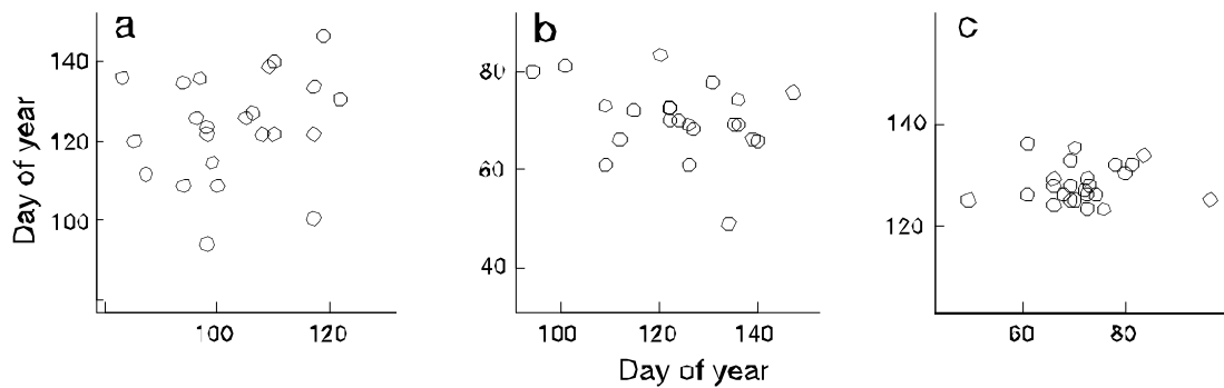
Fig. S2. Three examples of the lack of relationship between the phenology of predators and prey. In all cases the upper trophic level is shown on the y -axis and the lower trophic level on the x -axis for: (a) peak copepod nauplii abundance date regressed against peak phytoplankton colour index date; (b) sandeel mean hatch date against copepod nauplii peak abundance date; (c) guillemot median egg laying date against sandeel mean hatch date (dates as day of year)
