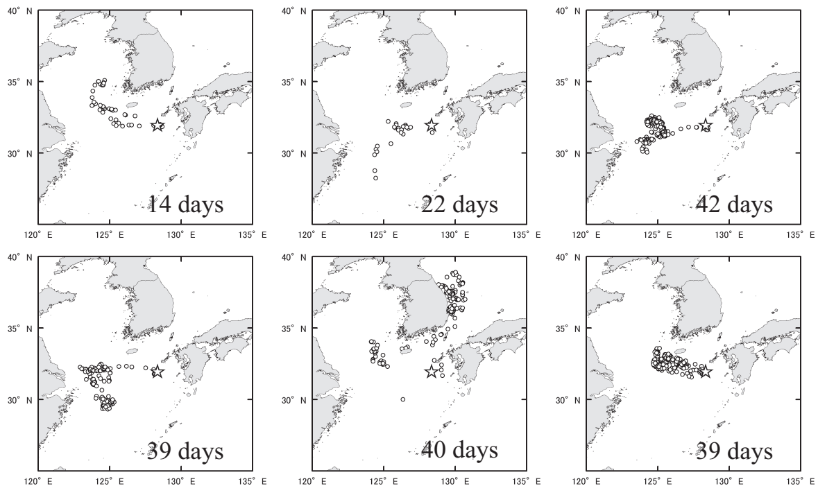
Fig. S1. Calonectris leucomelas . Individual tracking maps of streaked shearwaters during the chick-rearing period from 8 September 2010 (next day of the GPS deployment) until the start of migration (18–21 October). Days tracked for each individual are shown.
