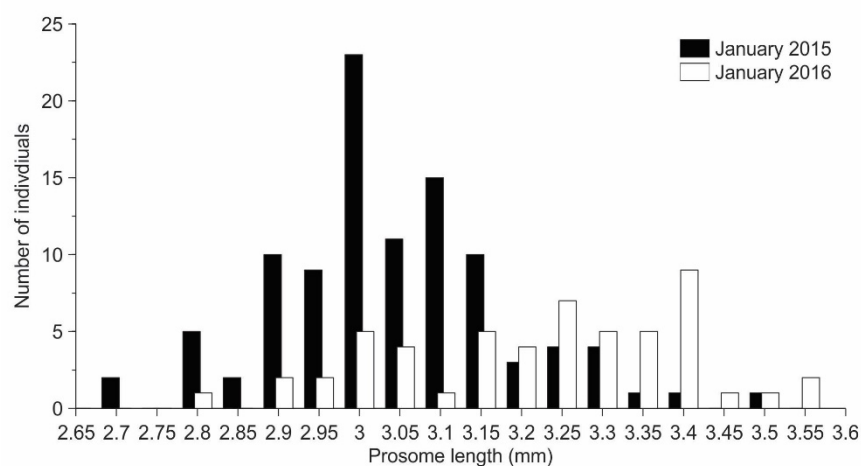
Fig. S1. Prosome length frequency distribution of Calanus females bearing spermatophores January 2015 (only KF) and 2016 (all fjords)
