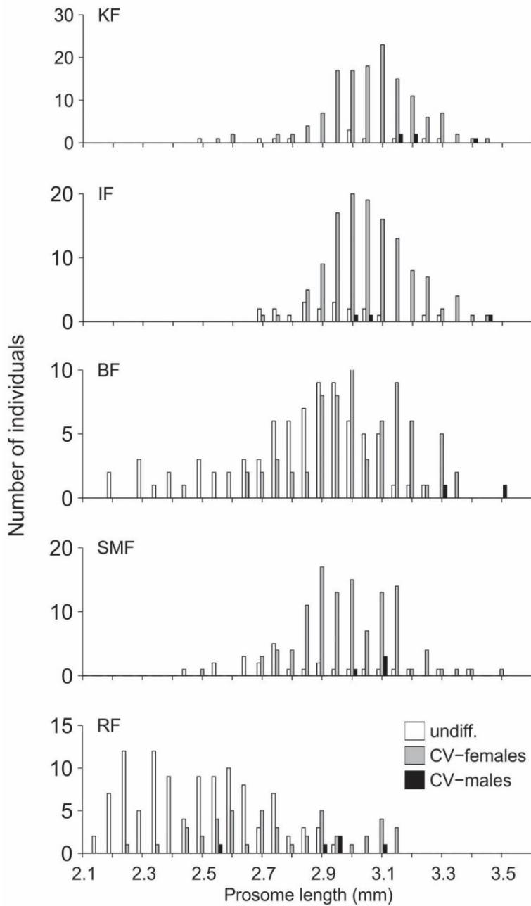
Fig. S2. Prosome length frequency distribution of Calanus copepodite stage CV ( C. finmarchicus and C. glacialis pooled) with sexually undifferentiated, female or male gonads from Kongsfjorden (KF), Isfjorden (IF), Billefjorden (BF), Smeerenburgfjorden (SMF) and Rijpfjorden (RF) in January 2016.
