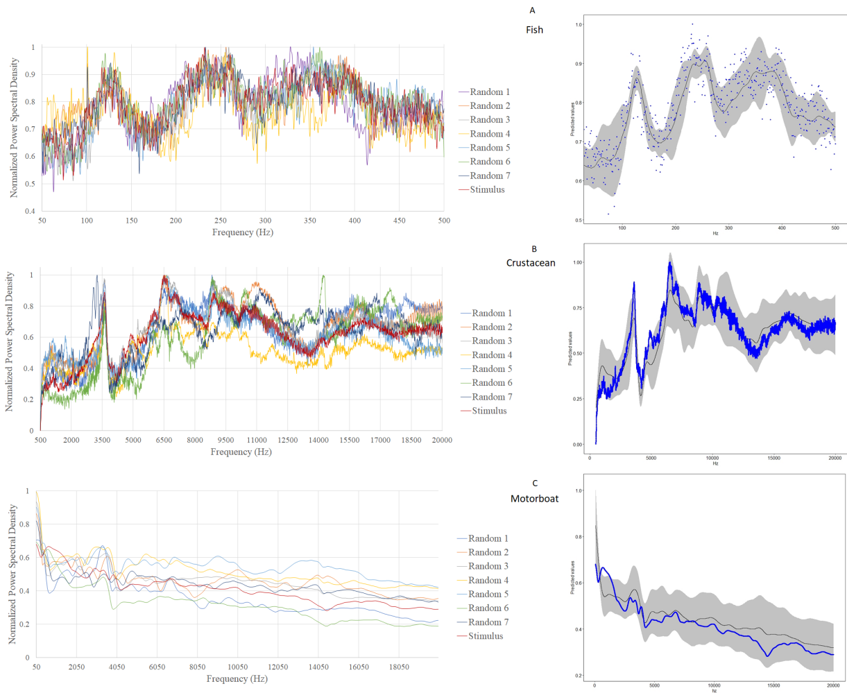
Fig. S1. Left: normalized Power Spectral Density (PSD) of A) fish, B) crustacean and C) motorboat stimuli used in the experiment and seven randomly selected 7-seconds files (random 1-7 containing fish/crustacean/motorboat sounds) from the entire dataset of the lagoon soundscape (Ceraulo et al. 2020). Right: comparison of the A) fish, B) crustacean and C) motorboat stimuli used in the experiment (represented in blue), the 95% confidence intervals (grey area) and the mean (black line) for the fitted GAM of the random selected stimuli.
