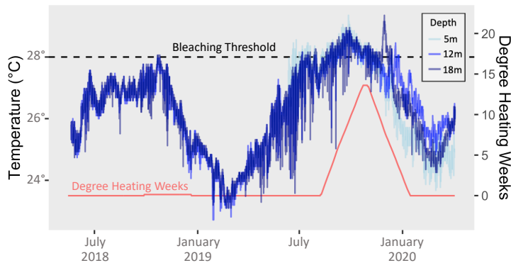
Fig. S2. Water temperature profiles at 5m (deployed June 2019), 12m (deployed May 2018), and 18m (deployed May 2018) covering the depth gradient of the Waikiki study site. Little bleaching was observed in 2018 when water temperatures did not rise above 28°C NOAA Bleaching Threshold (dashed line). In 2019, water temperature initially rose above 28°C in July and consistently remained above 28°C from 5 September through 31 October and again from 25 November to 12 December.
