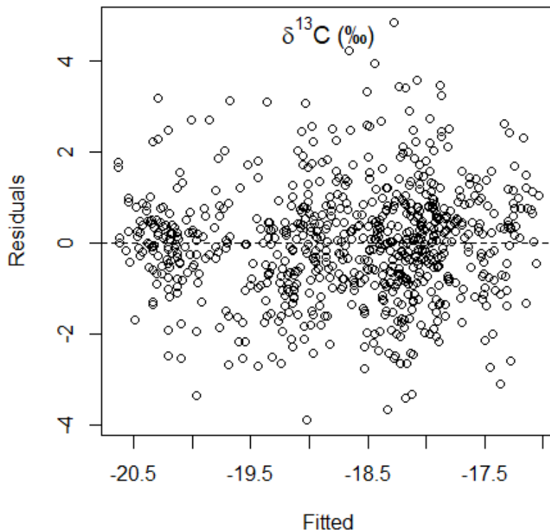
Figure S1. Model validation for the optimum generalized additive mixed models applied to the response variable C ( \delta^{13}\text{C} ). Fitted values were plotted against residuals to ensure no residual patterns were evident.
