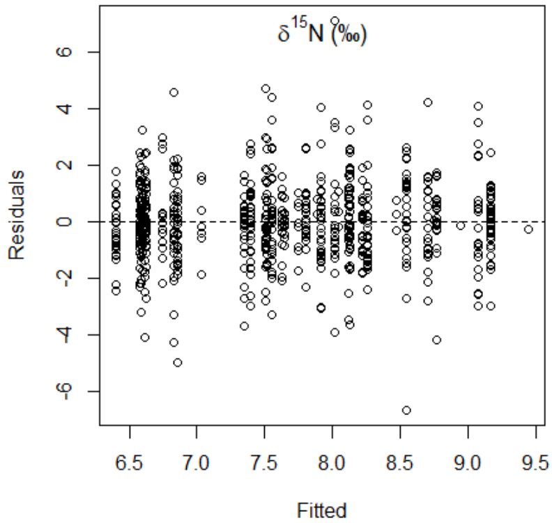
Figure S2. Model validation for the optimum generalized additive mixed models applied to the response variables N ( \delta^{15}\text{N} ). Fitted values were plotted against residuals to ensure no residual patterns were evident.
