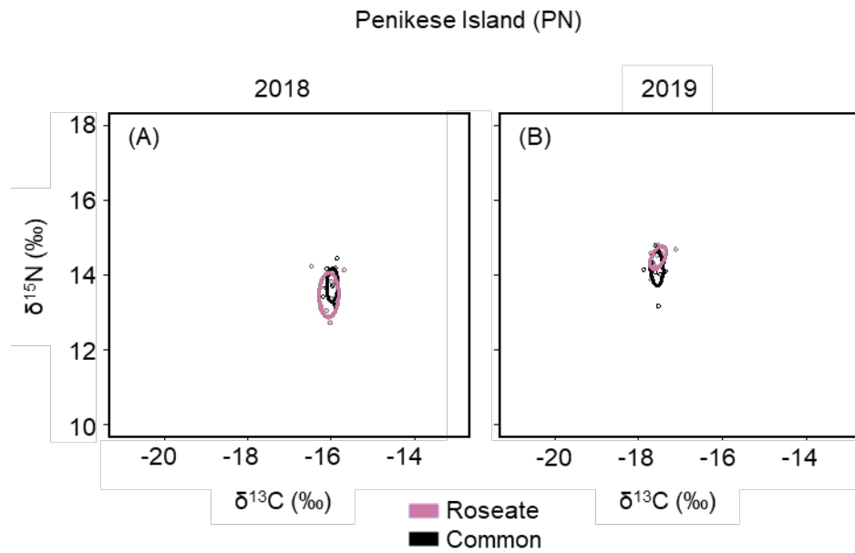
Fig. S7. Estimated standard ellipses showing isotopic niches for the eggshells of roseate terns (pink) and common terns (black) nesting on Penikese Island in 2018 (A) and 2019 (B).
